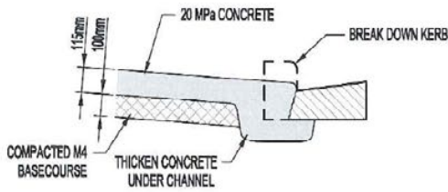
CHANNEL DETAIL
